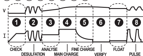
Phases de la charge PULSE-TRONIC.
