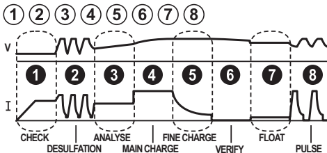
Fasi carica PULSE-TRONIC.
